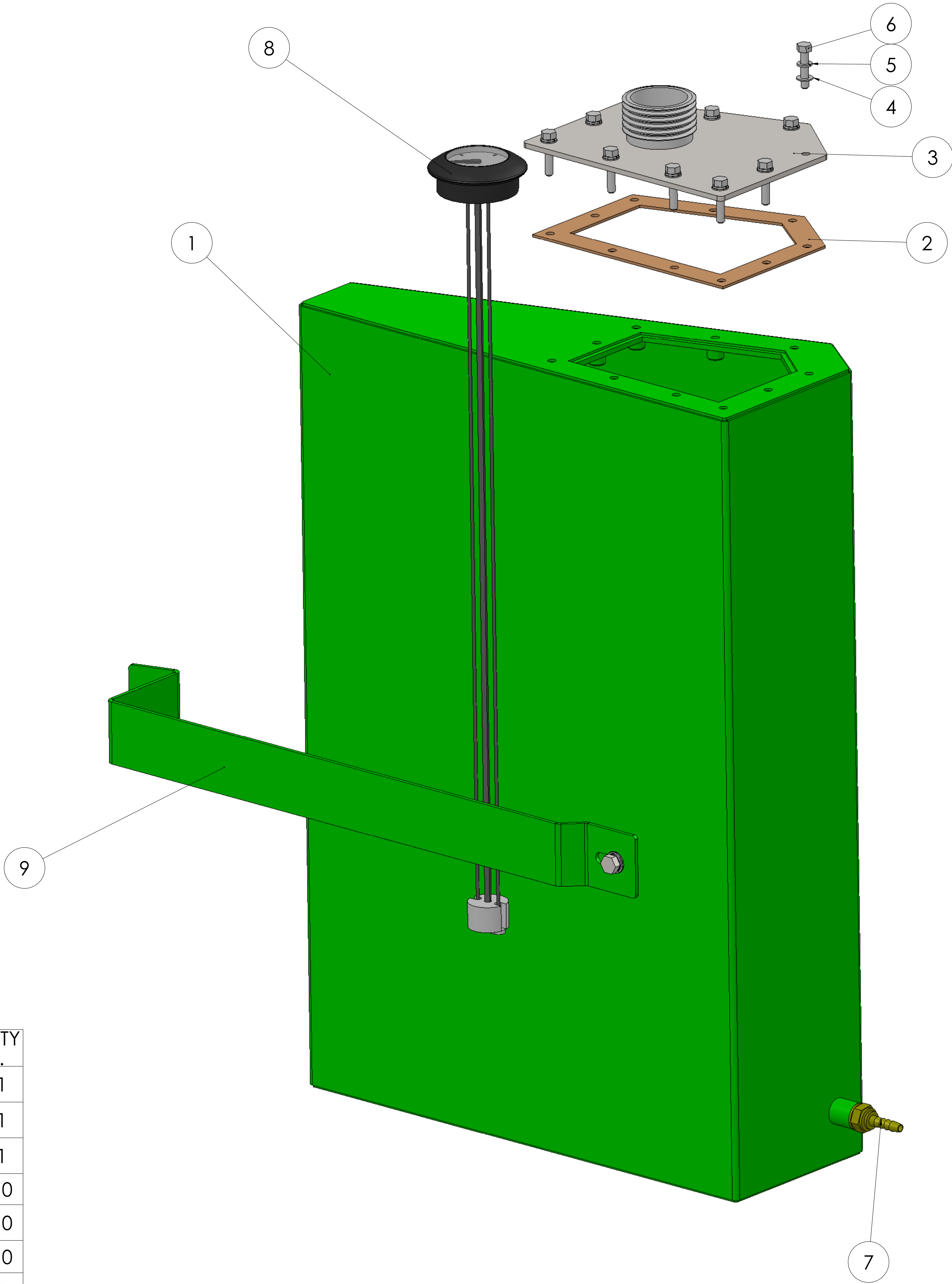
STEEL TANK FOR PETROL MACHINES
